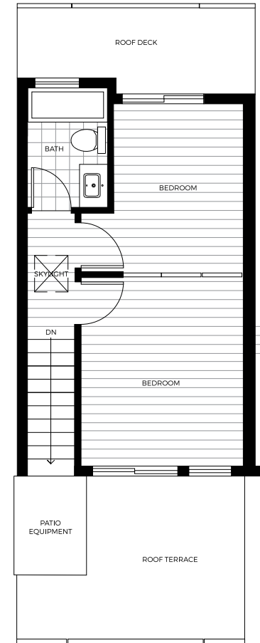
4th LEVEL
